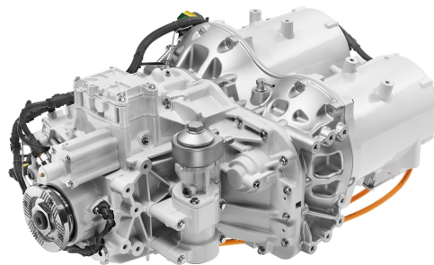
Volvo FE engine 370kW/850NM
