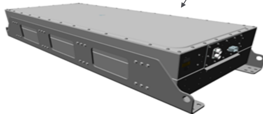
Battery Lithium-ion 2-6, 50kWh/520kg Range 200-300km Charge time 1-2h or 10h
